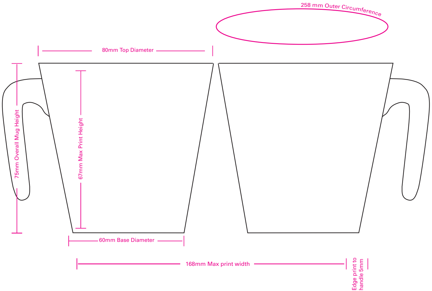
MUG PRINT AREA AFTER ARCING TO SHAPE OF MUG
